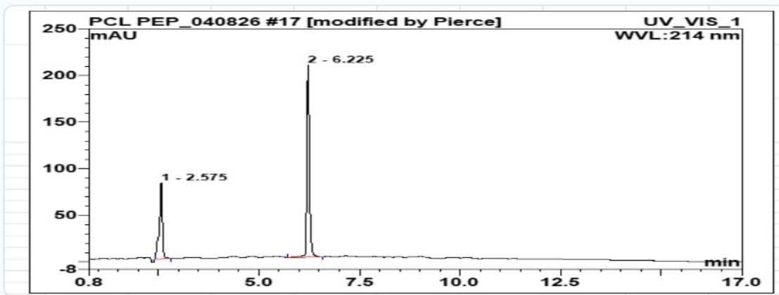
HPLC Chromatogram (Retention Time: 2.575, 6.225 min)
